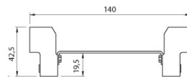
5122/314
