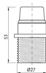
D/3350
