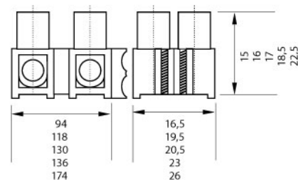
T55/T85
