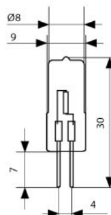
JC-G4
