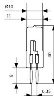
JC-GY6,35
